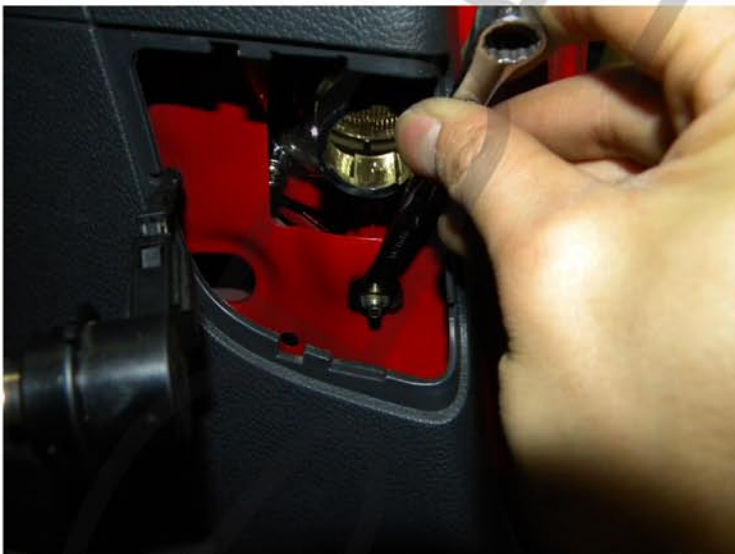
3. Remove two 10mm bolts then remove the trunk taillight
