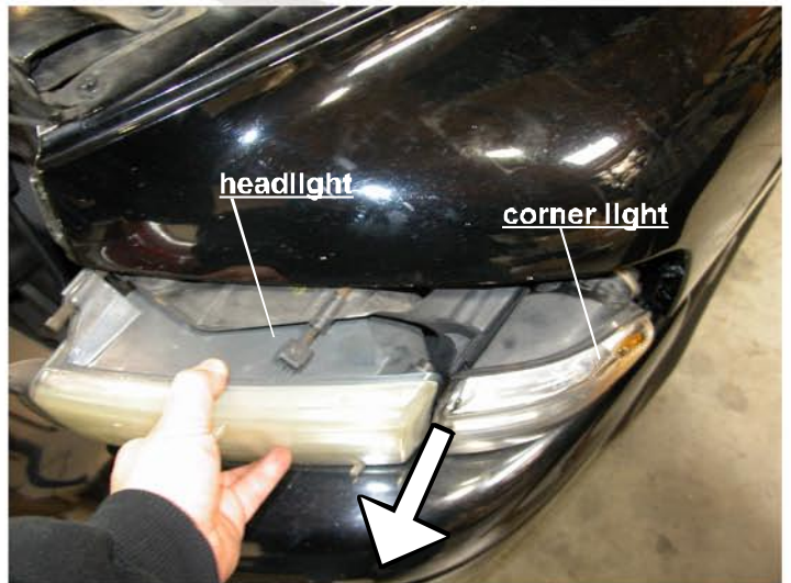
4. Pull out the headlight a little bit first (BOTH SIDE)
