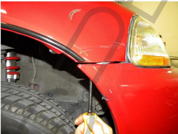
3. Remove the screw that connects the fender and front bumper
