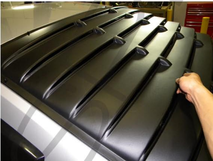
9. Carefully position the louver onto the rear window
