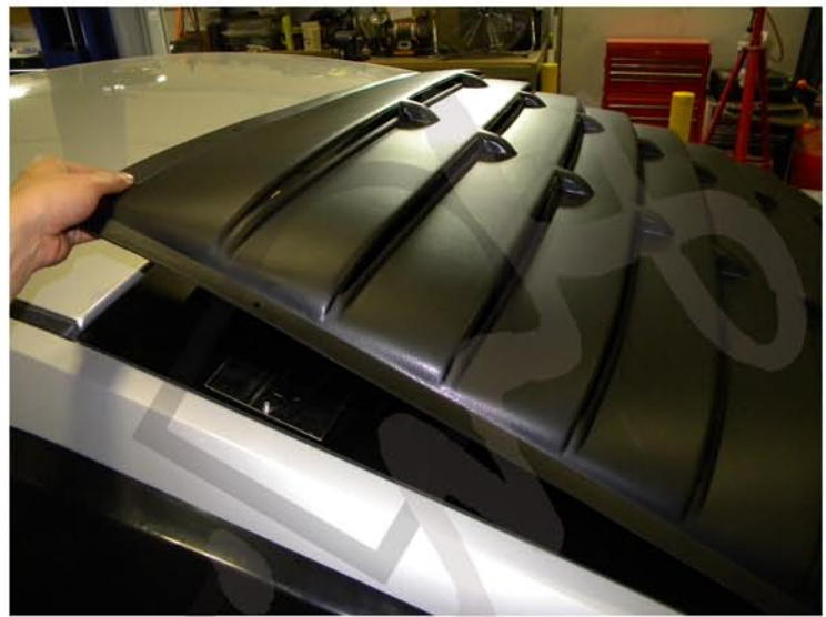
12. Lift the louver off of rear window with bracketing still attached
