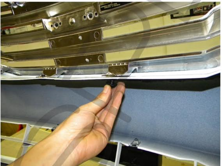
15. Secure grill with 4 plastic clips
