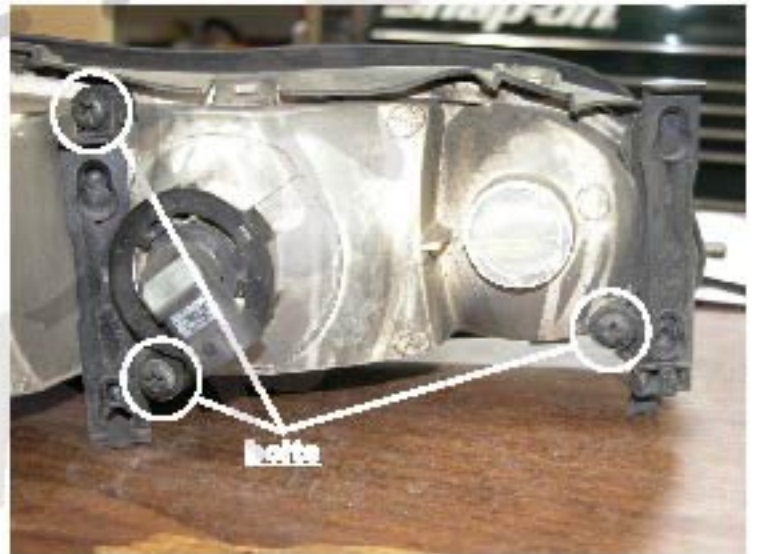
8. After you disconnect all the connectors from the headlight, it should look the same as the picture shown above, also there are three bolts in the back of the headlight
