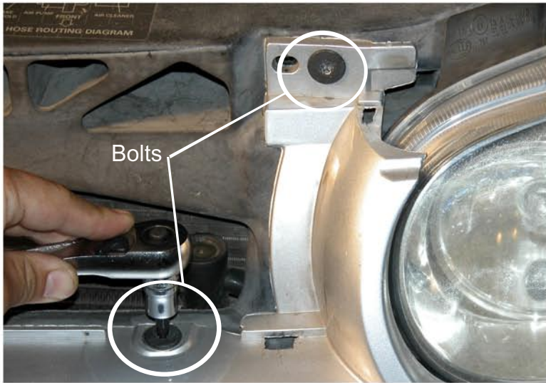
5. After you remove the grill, next use the T30 torx socket to remove the two bolts
