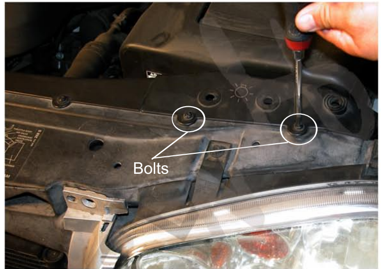
6. Use philip screwdriver to remove the two bolts to unlock the headlight wire cover
