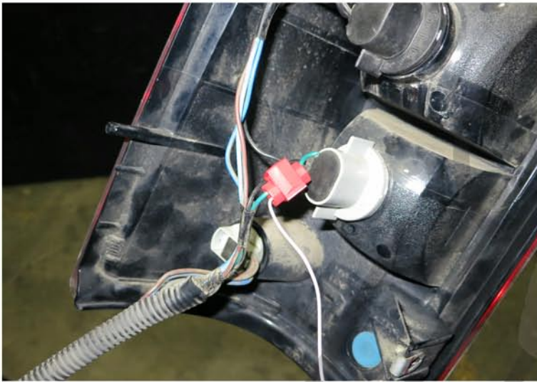
7. Connect the white wire to the reverse light positive wire with the quick connector
